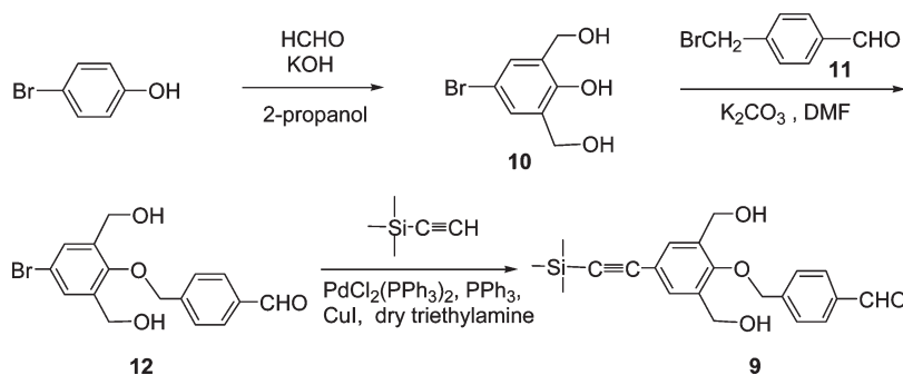
Scheme 2. Synthetic Route to Compound 9
