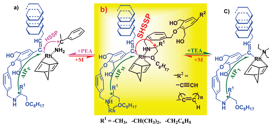
Figure 8. Three mechanisms (HSSP, SHSSP, and AIP) of asymmetric polymerizations of ORDHPAs having a chiral bidentate ligand by using achiral and chiral catalytic systems. (a) HSSP by using ( R )-PEA. (b) SHSSP by using no cocatalysts. (c) AIP by using TEA.
