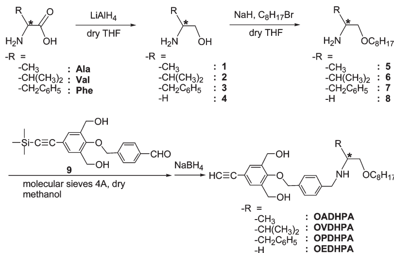
Scheme 1. Synthetic Route to ORDHPAs (OADHPA, OVDHPA, OPDHPA, and OEDHPA)
